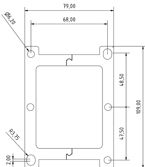
INTEL LGA 3647 Narrow
