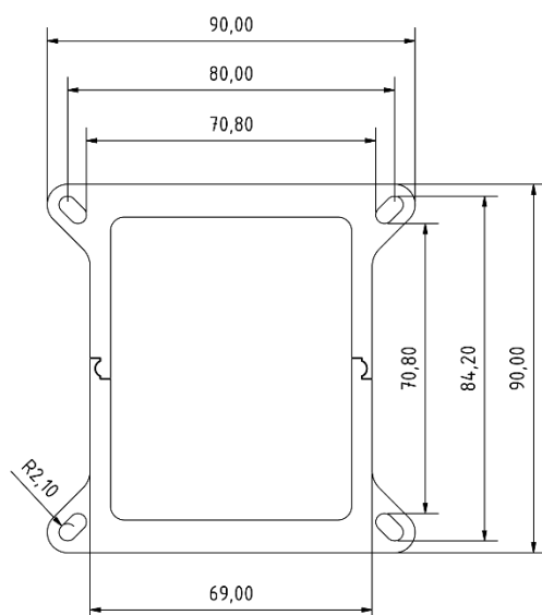
INTEL LGA 2066 LGA 2011
